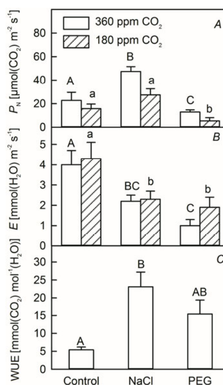
Fig. 2. Effect of osmotic (PEG) and salt (NaCl) treatments on (A) net photosynthetic rate ( P_N ), (B) transpiration rate ( E ), and (C) water-use efficiency (WUE) of Haloxylon aphyllum shoots. The values are means ( \pm SD) of four replicates. The various capital and lowercase letters indicate a significant difference at P < 0.05 (Tukey's pairwise comparison) under different CO 2 concentrations.
